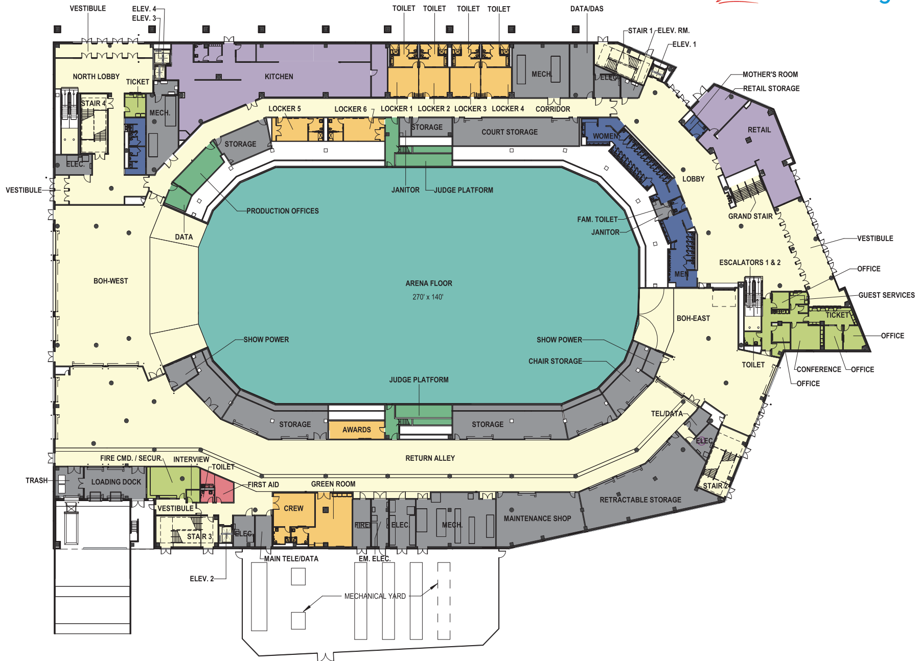
EVENT LEVEL PLAN
